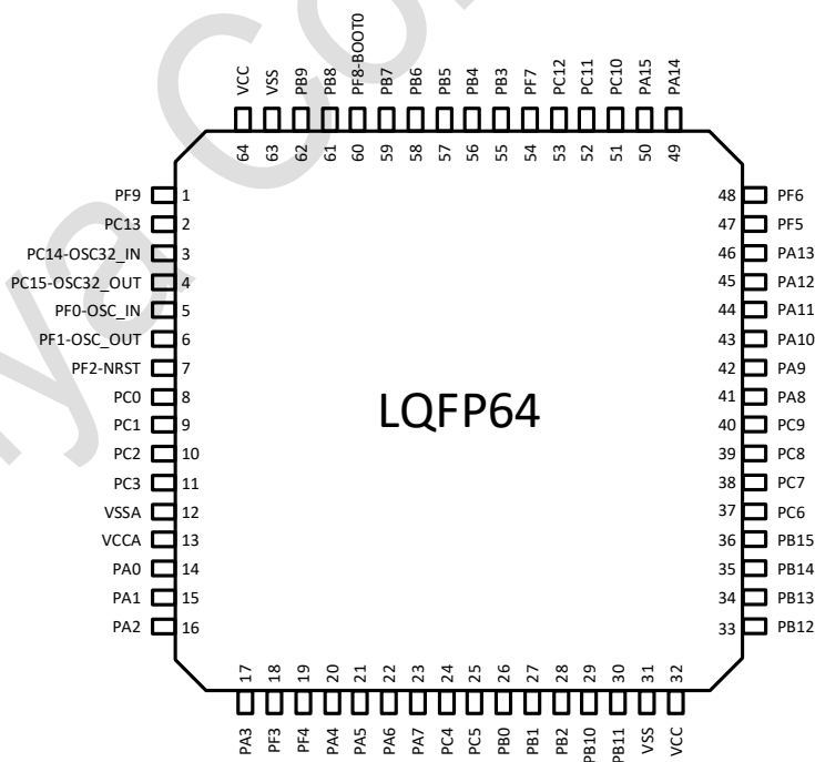
Figure 3-2 LQFP64(12*12) PY32F040R2xT6 Pinout2(Top view)
