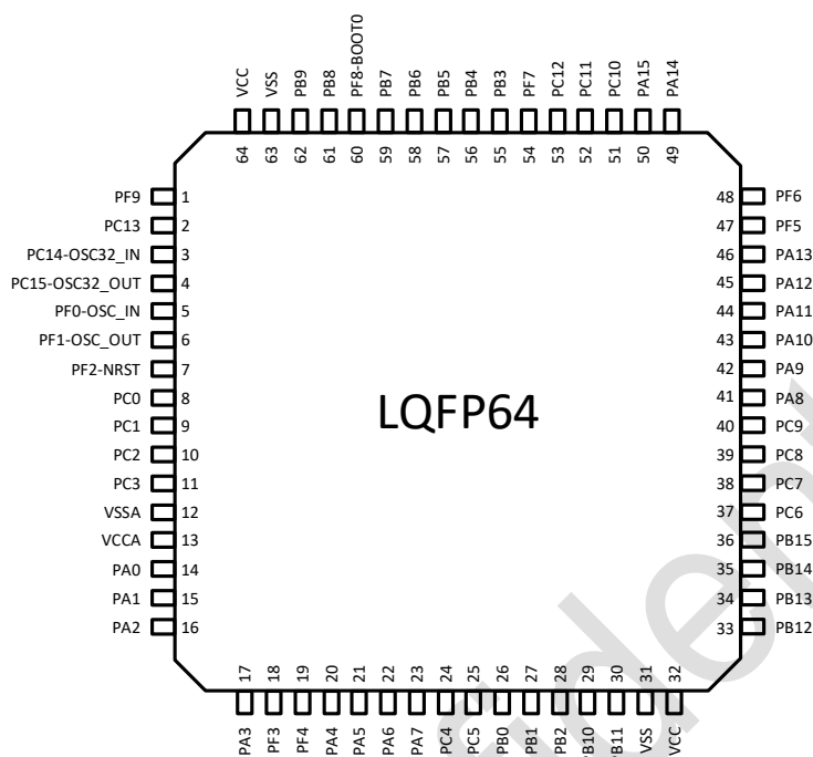
Figure 3-1 LQFP64(10*10) PY32F040R1xT6 Pinout1(Top view)
