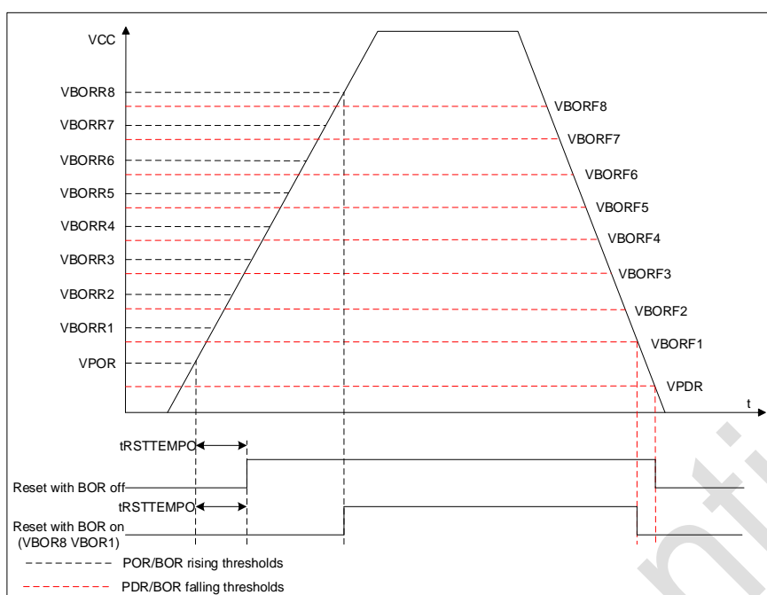
Figure 2-3 POR/PDR/BOR threshold
